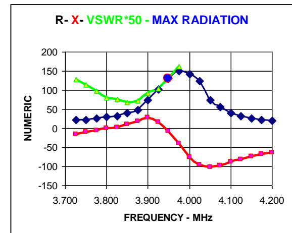
FIGURE 11 – BEFORE ADDING THE SOURCE COIL
