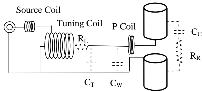
SCHMATIC DIAGRAM
