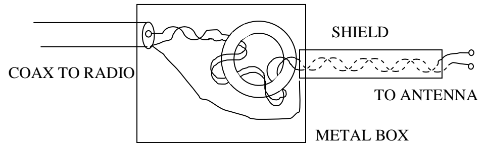
FIGURE 13 – CURRENT BALUN
