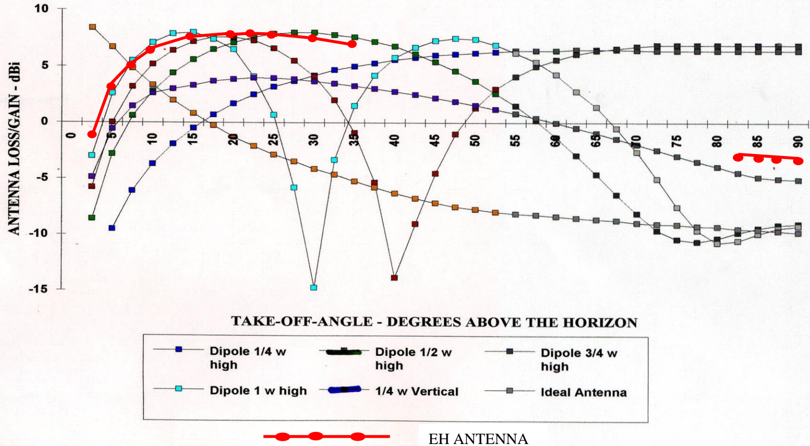
FIGURE 6 – RADIATION PATTERNS OF VARIOUS ANTENNAS
