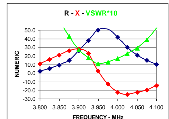
FIGURE 12 – IMPEDANCE AFTER ADJUSTING THE SOURCE COIL
